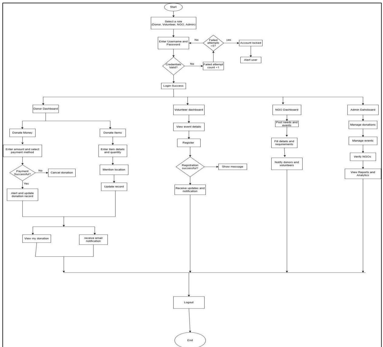
Figure 4: Flowchart
