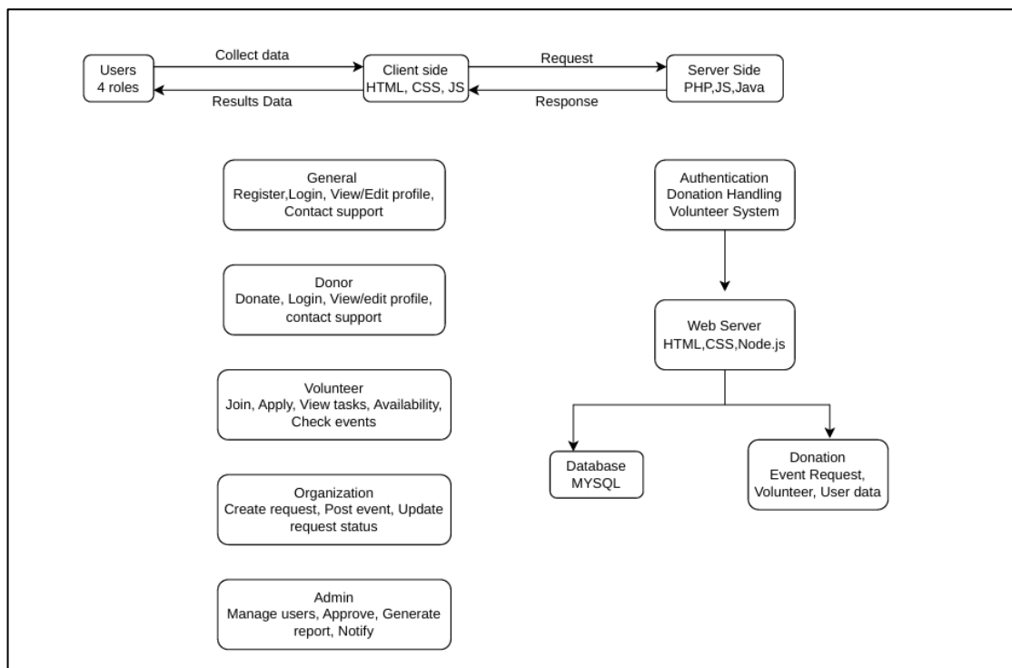
Figure 5: System Architecture
