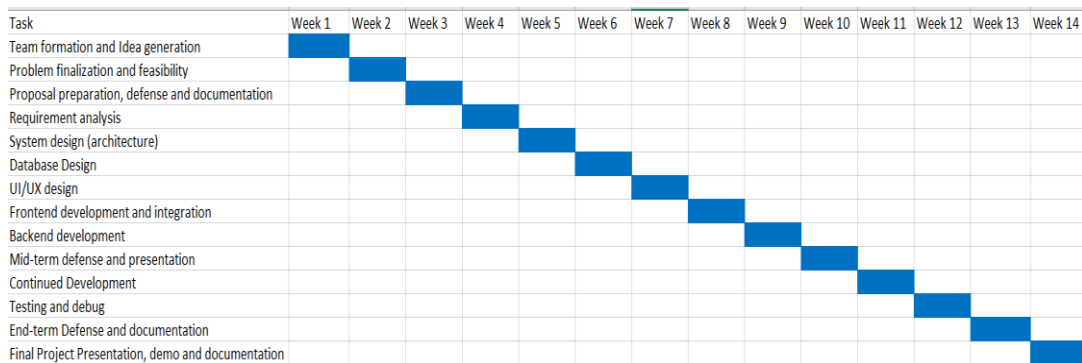
Figure 2: Gantt Chart
